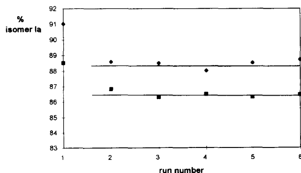
Fig. 1. Stability of the polyamide (2,6-py series)-bound catalysts \text{Rh-3} (♦) and \text{Rh-4} (■) during recycling tests (hydrosilylation of isoprene by \text{Me}_2\text{PhSiH} ).
