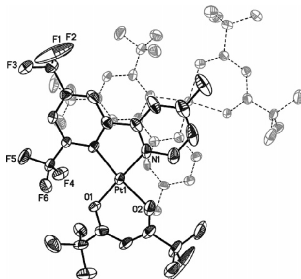
Figure 4. ORTEP drawing of the \pi - \pi stacked platinum complex 10 . This is an example of the classical twisted phenyl-pyridine alignment in \pi - \pi stacking. The plane-to-plane distance is 3.478 Å. The Pt-Pt distance is 5.084 Å.
