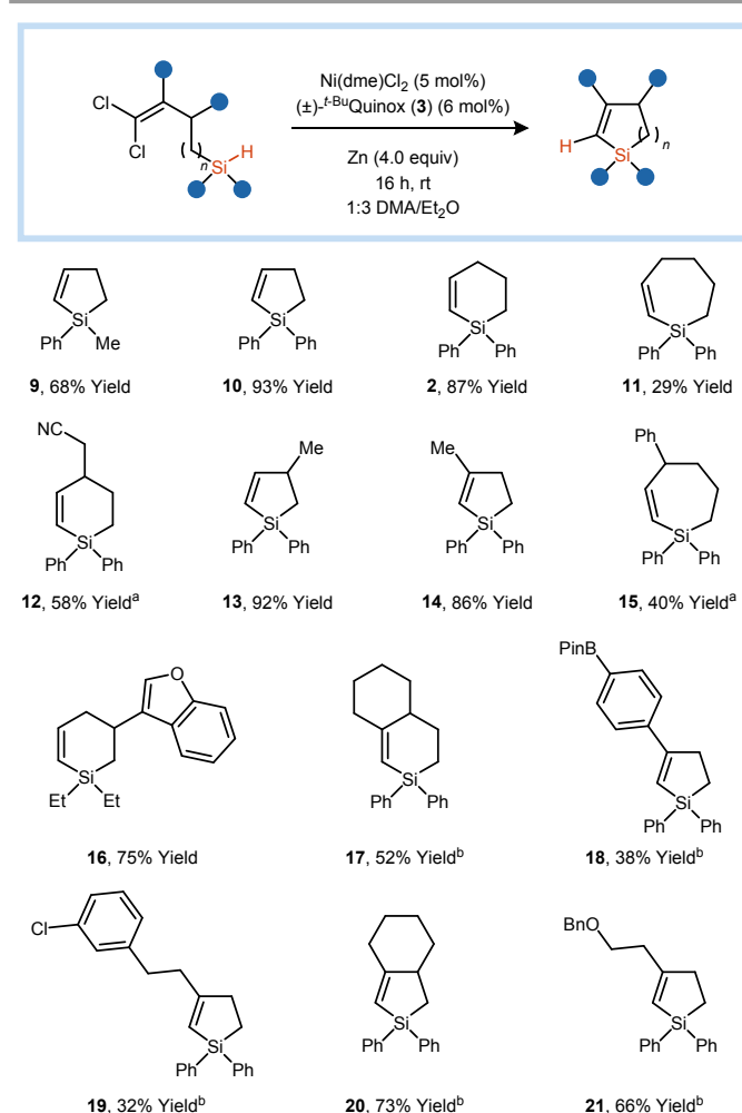
Figure 2. Substrate scope studies. Reactions were conducted using the standard conditions shown in Table 1. a 10 mol% catalyst loading. b 20 mol% catalyst loading; 50 °C temperature
