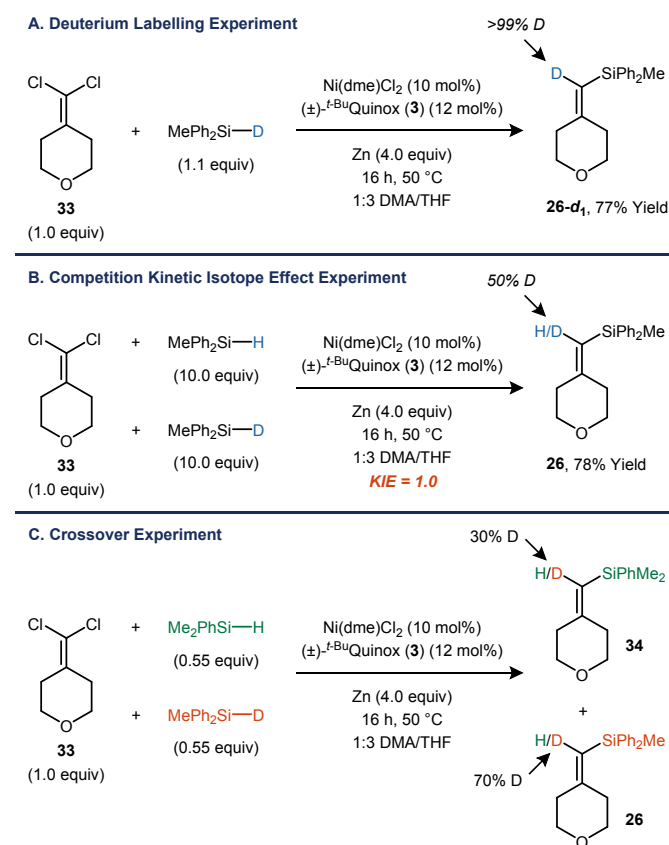
Figure 4. Mechanistic studies using a deuterium-labelled silane.
