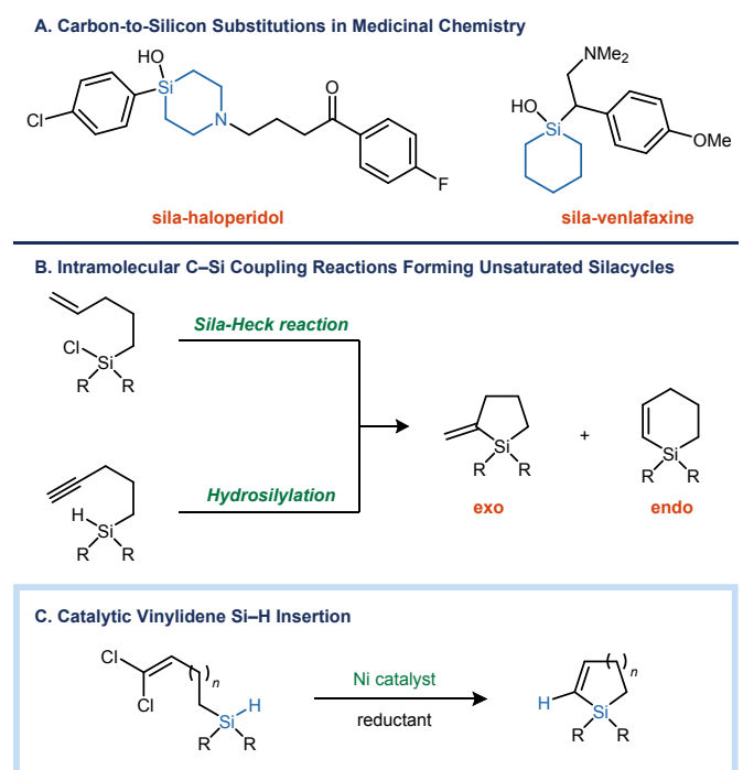
Figure 1. Nickel-catalyzed reductive insertions of 1,1-dichloroalkenes into Si–H bonds as a route to unsaturated silacycles.
