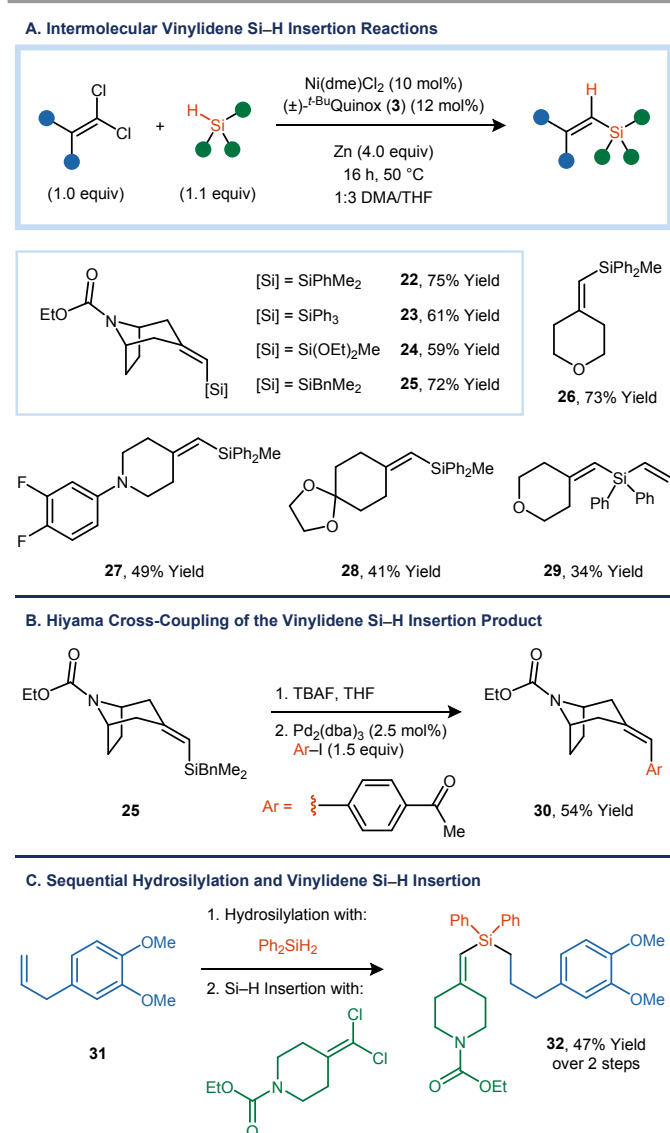
Figure 3. (a) Intermolecular vinylidene Si–H insertion reactions, providing trisubstituted vinylsilanes. (b) Synthesis of a vinylsilane that can be utilized as a nucleophilic partner in a Hiyama cross-coupling reaction. (c) Sequential hydrosilylation and vinylidene Si–H insertion reactions of a secondary organosilane.
