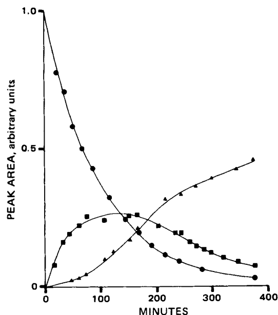
Figure 2—Time course for chlorambucil and degradation products in aqueous solution. Key: ●, chlorambucil (A, Scheme I); ■, I (C, Scheme I); and ▲, 4-[p-[di(2-hydroxyethyl)amino]phenyl]butyric acid (E, Scheme I). The molar absorbance and yield from the chromatographic column were considerably lower for E compared to A and C.
