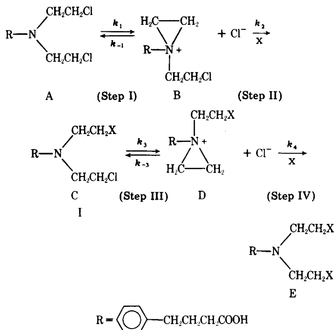
Scheme I—Degradation of nitrogen mustards
