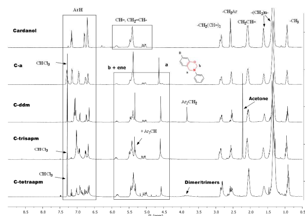
Figure 2. ^1\text{H} -NMR spectra of cardanol and Bz monomers in \text{CDCl}_3 .
