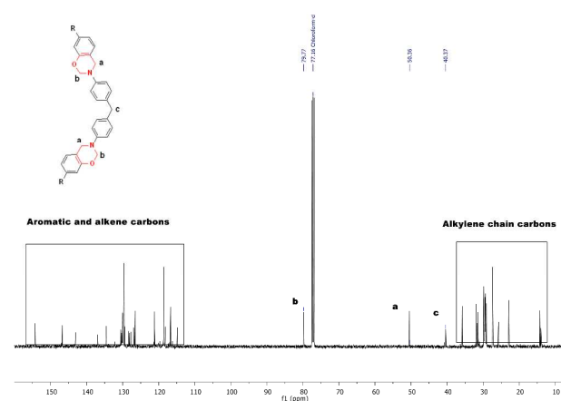
Figure 3. ^{13}\text{C} -NMR spectrum of C-ddm in \text{CDCl}_3 .
