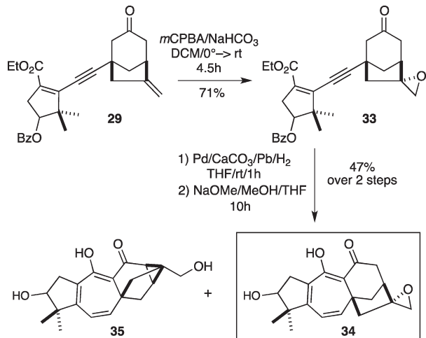
Scheme 6. Optimized Reduction/Cyclization Giving Advanced Intermediate 34 toward a Total Synthesis of Pierisformaside C ( 1 )
