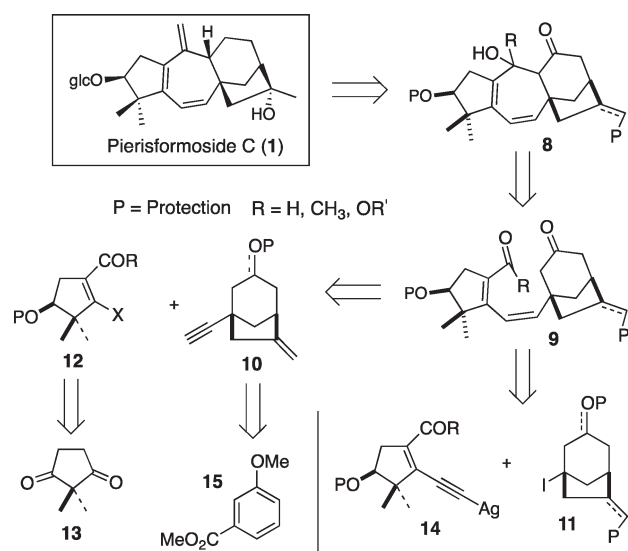
Scheme 1. Retrosynthetic Analysis for Pierisformaside C ( 1 )
