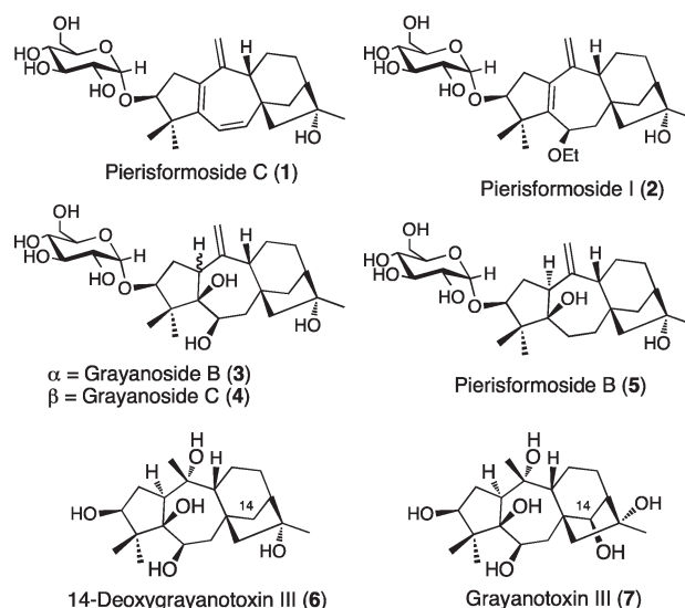
Figure 1. Diterpene glucosides 1 – 5 and grayanotoxins 6 and 7 .
