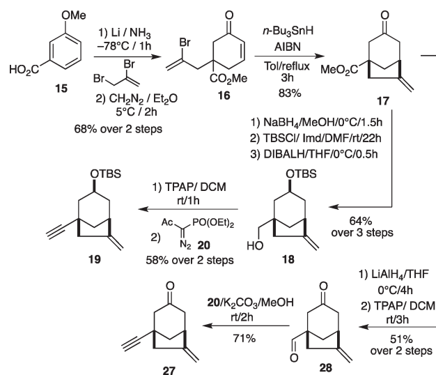
Scheme 2. Synthesis of Bicyclo[3.2.1]octane Derivatives 19 and 27
