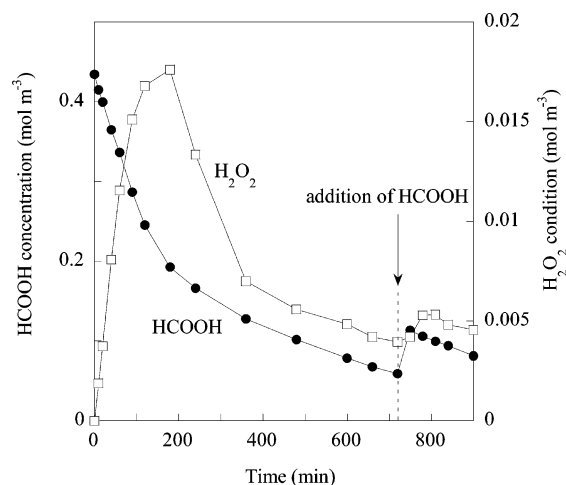
Figure 8. Time courses of HCOOH and \text{H}_2\text{O}_2 concentrations in treatment of a 3.0 \times 10^{-4} \text{ m}^3 aqueous solution of HCOOH at an initial concentration of 0.45 \text{ mol m}^{-3} by \text{TiO}_2 under irradiation with UV light from a blacklight blue fluorescent lamp. A 5.0 \times 10^{-5} \text{ m}^3 aqueous solution of HCOOH at 0.45 \text{ mol m}^{-3} was added after 720 min.
