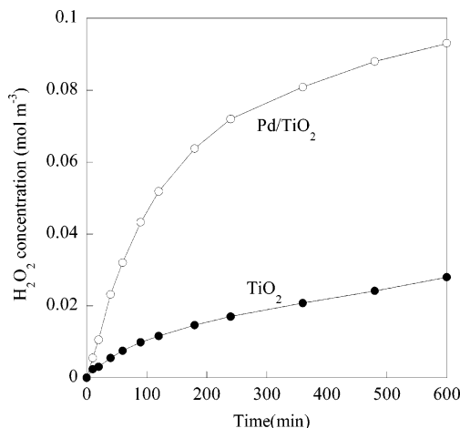
Figure 6. Formation of \text{H}_2\text{O}_2 from water by photocatalyst under irradiation with UV light from a germicidal lamp.
