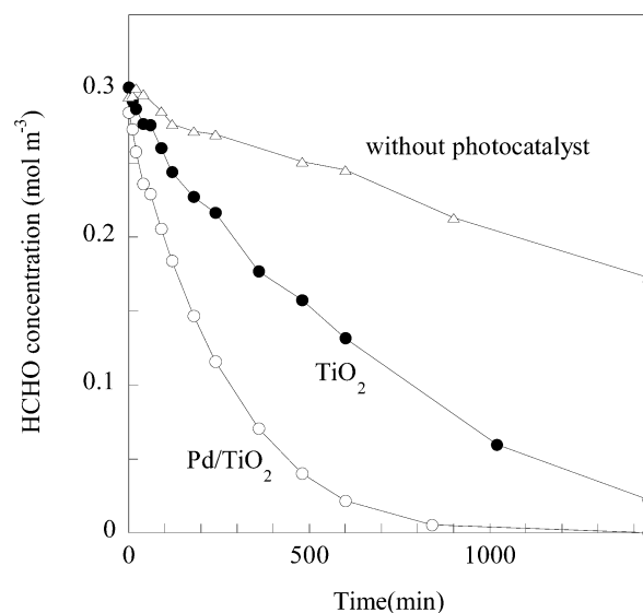
(a) Change in HCHO concentration
