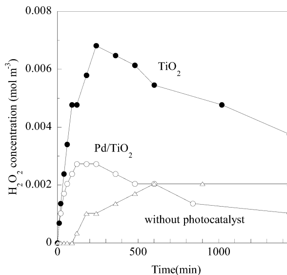
(b) Change in \text{H}_2\text{O}_2 concentration
