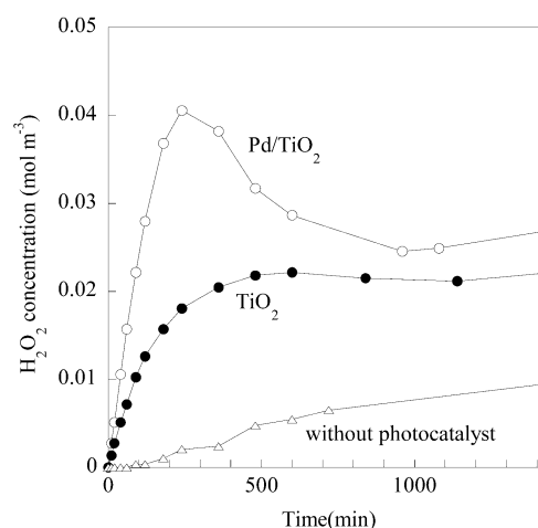
(b) Change in \text{H}_2\text{O}_2 concentration
