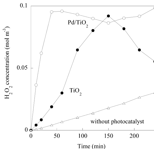
(b) Time courses of H 2 O 2 concentration
