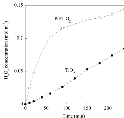
Figure 11. Time courses of H 2 O 2 concentration under irradiation of water with UV light from a germicidal lamp.
