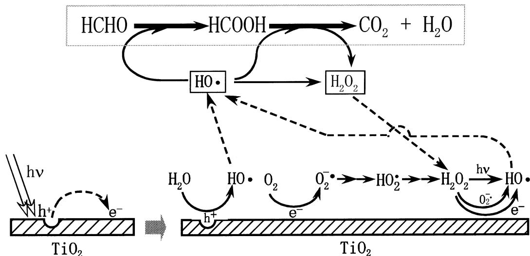
Figure 15. Reaction mechanism proposed for photocatalytic decomposition of HCHO.
