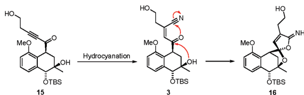
Scheme 4. Plausible Mechanism for the Formation of the Imideate 16 from Alkynone 15
