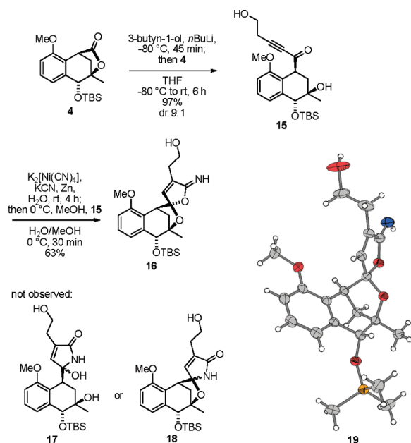
Scheme 3. Nickel(0)-Mediated Hydrocyanation Leading to the Formation of the Cyclic Imideate 16
