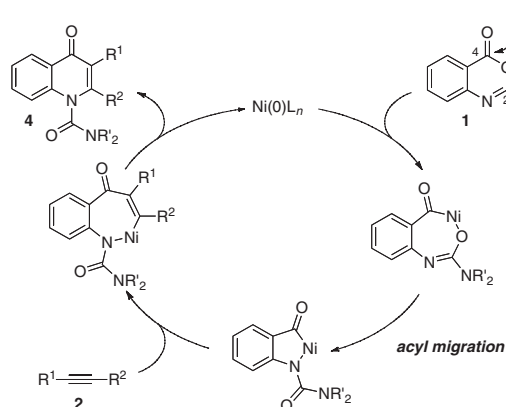
Scheme 5. Plausible reaction mechanism.
