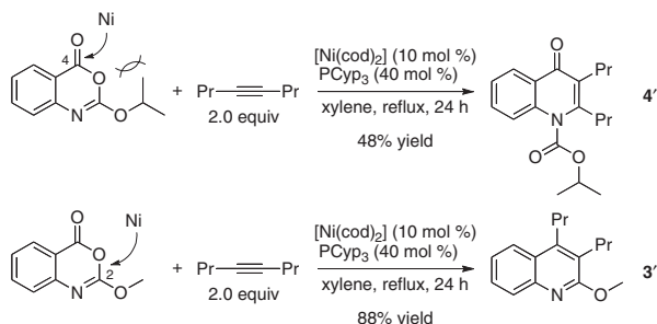
Scheme 4. Effects of substituent.
