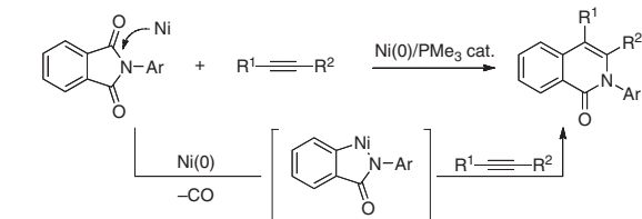
Scheme 1. Cycloaddition of N -arylphthalimides with alkynes.
