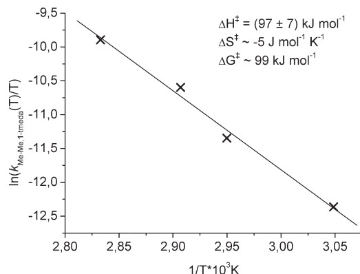
Figure 1. Eyring plot of second-order rate constants k_{\text{Me-Me}, 1\text{-tmEDA}}(T) for the decomposition of 1 -tmEDA to \text{C}_2\text{H}_6 in \text{dmsO-d}_6 solution (as determined from the decrease of the total \text{Ni(II)-CH}_3 integral in the temperature range from T = 55 to 80^\circ\text{C} ).
