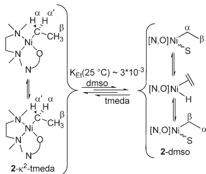
Scheme 3. Dynamic Processes of 2-dmsO and 2- \kappa^2 -tmeda Observed by 2D ROESY at T = 25^\circ\text{C}
