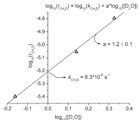
Figure 4. Concentration dependence of observed initial rates of hydrolysis r_{\text{CH}_3\text{D}} on added water as a plot of \log_{10}(r_{\text{CH}_3\text{D}}) vs \log_{10}([\text{D}_2\text{O}]) ( 1 -tmeda] t=0 = 34 mM, [\text{D}_2\text{O}] = 0.69, 1.38, and 2.12 M, T = 55 °C).
