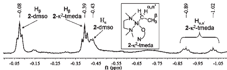
Figure 2. Typical high-field ^1\text{H} NMR chemical shift region of Ni(II)-alkyls 2-dmsO and 2- \kappa^2 -tmeda prepared in an NMR tube in \text{dmsO}-d_6 at T = 55^\circ\text{C} (spectrum shown acquired at 25^\circ\text{C} ).
