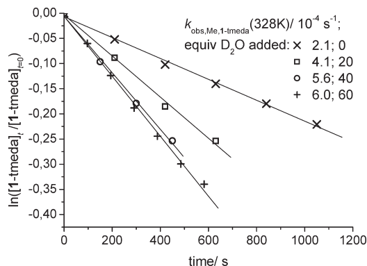
Figure 3. Pseudo-first-order plots of the time-dependent decrease of 1 -tmeda in the presence of ethylene and 0 to 60 equiv of D 2 O (pseudo-first-order rate constants k_{\text{obs,Me,1-tmeda}} determined by linear regression); 34 mM 1 -tmeda, \sim 0.1 M ethylene.
