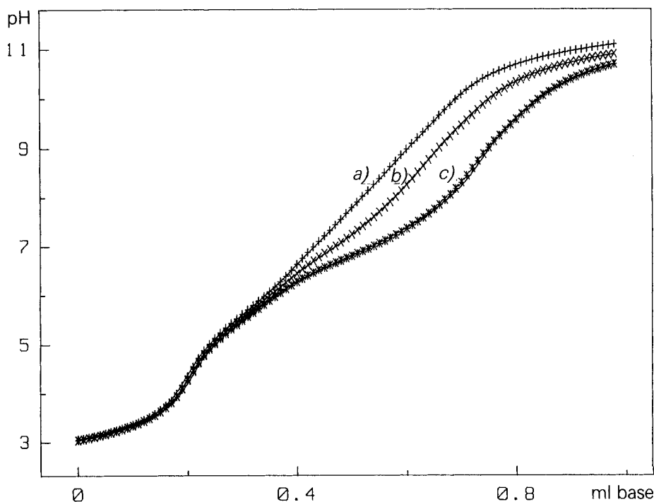
Fig. 3. Potentiometric titration curves of 1 ( 5.5 \cdot 10^{-4} M) with a) 45%, b) 90%, and c) 180% \text{Ca}^{2+} in 0.1 M \text{Me}_4\text{N}(\text{NO}_3) at 25°. Titrating base, 0.1 M \text{Me}_4\text{N}(\text{OH}) .
