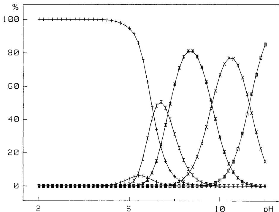
Fig. 4. Species distribution for 5.5 \cdot 10^{-4} M 1 and 4.95 \cdot 10^{-4} M \text{Ca}^{2+} calculated with the stability constants of Table 3. \text{Ca}^{2+} (+), [\text{CaLH}_4]^{2-} (I), [\text{Ca}_2\text{LH}_2]^{2-} (II), [\text{Ca}_2\text{LH}]^{3-} (*), [\text{Ca}_2\text{L}]^{4-} (x), [\text{CaL}]^{6-} ( \Phi ).
