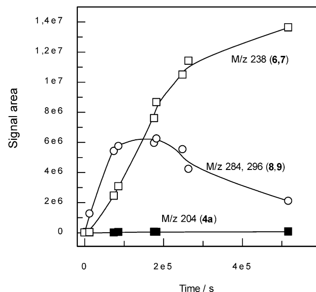
Fig. 3 Time-dependent product distribution for the reaction of 9-ethylguanine ( 1a ; <0.5 mmol dm -3 ) with BMA at pH 5.3 and 60 °C. Notation: 1, N 2 -( trans -1,2-dihydroxyethano)-9-ethylguanine ( 6 , □), 1, N 2 -(1,2,2,4-tetrahydroxypropano)-9-ethylguanine and 1, N 2 -(2-formyl-1,2,3-trihydroxypropano)-9-ethylguanine ( 8 + 9 ; ○) and N 2 ,3-etheno-9-ethylguanine ( 4a ; ■).
