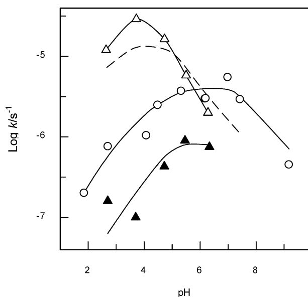
Fig. 1 pH-Rate profiles for the reactions of various 9-substituted guanines ( < 0.5 \text{ mmol dm}^{-3} ) with BMA ( 10 \text{ mmol dm}^{-3} ) at 60^\circ\text{C} . Notation: 9-ethylguanine ( 1a ; \circ ), 9-ethyl- O^6 -methylguanine ( 2 ; \Delta ), 9-ethyl-1-methylguanine ( 3 ; \blacktriangle ). The dotted line refers to the reaction of 9-methyladenine with BMA. 18
