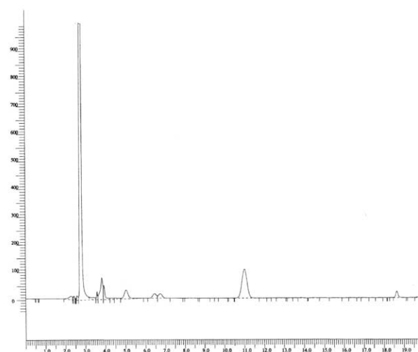
Fig. 4 RP-HPLC chromatogram of the reaction mixture of 2'-deoxyguanosine ( 1b ; <0.5 mM) with BMA (10 mM) at pH 7.4 and 60 °C. Annotation: t R 5 min: 1, N 2 -(1,2,2,4-tetrahydroxypropano)-2'-deoxyguanosine and 1, N 2 -(2-formyl-1,2,3-trihydroxypropano)-2'-deoxyguanosine ( 8 + 9 ), t R 6–7 min 1, N 2 -(1,2-dihydroxyethano)-2'-deoxyguanosines ( 6 and 7 ), t R 11 min 2'-deoxyguanosine ( 1b ) and t R 19 min 1, N 2 -etheno-2'-deoxyguanosine ( 5b ).
