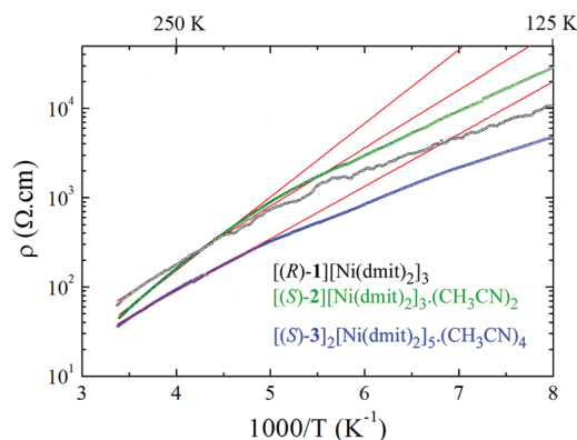
Figure 7. Temperature dependence of the resistivity of the three salts. Red line is a model in the high-temperature regime with \rho = \rho_0 \exp(E_{\text{act}}/kT) .
