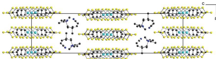
Figure 3. Projection view along the b axis of the unit cell of the 'Bu salt, [( S )-2][Ni(dmit) 2 ]·(CH 3 CN) 2 .
