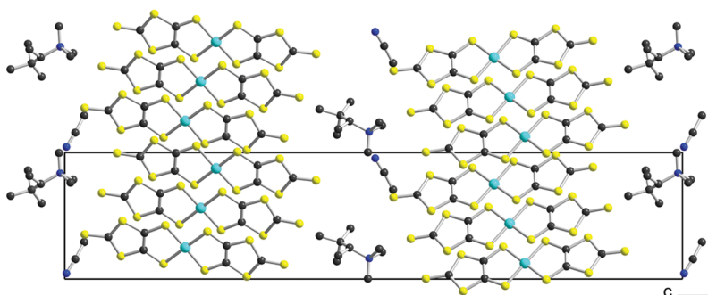
Figure 11. Projection view (along the a axis) of the unit cell of the monoclinic phase of [(rac)\text{-}2][\text{Ni}(\text{dmit})_2] \cdot (\text{CH}_3\text{CN})_2 .
