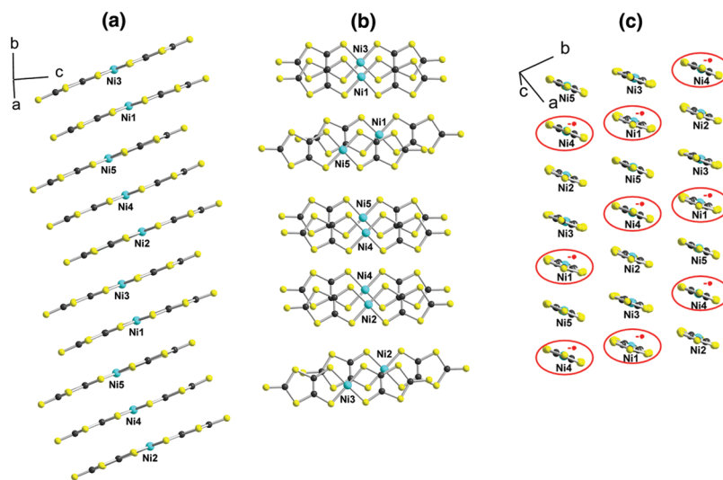
Figure 9. Structure of [(S)-3]_2[Ni(dmit)_2]_5 \cdot (CH_3CN)_4 with (a) detail of the alternating dimer and trimer structure of the stack of [Ni(dmit)_2] moieties, (b) the overlap patterns between molecules, and (c) the charge repartition deduced from comparison of intramolecular bond distances.
