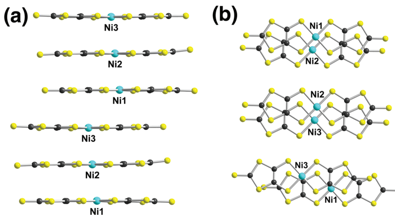
Figure 5. Detail of the trimerized stacks (left) and overlap patterns within stacks (right) in [(\text{S})-2][\text{Ni}(\text{dmit})_2]_3\cdot(\text{CH}_3\text{CN})_2 .
