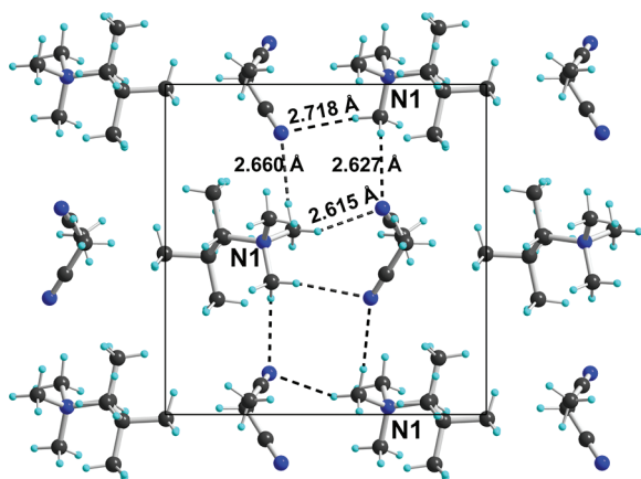
Figure 4. Weak \text{N}^+-\text{CH}_3\cdots\text{N}\equiv\text{C}-\text{CH}_3 hydrogen-bond network between the (S)-2 cation and \text{CH}_3\text{CN} molecules in [(\text{S})-2][\text{Ni}(\text{dmit})_2]_3\cdot(\text{CH}_3\text{CN})_2 .
