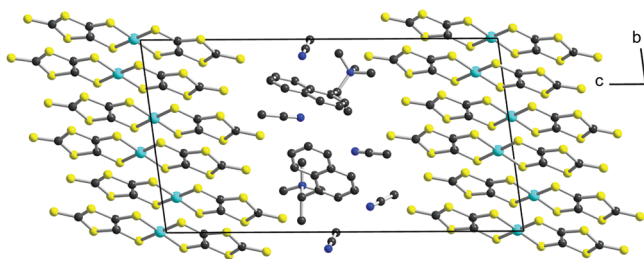
Figure 8. Projection view along the a axis of the unit cell of [(S)-3]_2[Ni(dmit)_2]_5 \cdot (CH_3CN)_4 .
