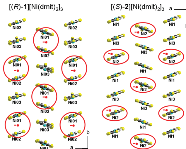
Figure 6. View of the slab built out of [\text{Ni}(\text{dmit})_2] species in [(\text{R})-1][\text{Ni}(\text{dmit})_2]_3 (left) and [(\text{S})-2][\text{Ni}(\text{dmit})_2]_3\cdot(\text{CH}_3\text{CN})_2 (right) with charge repartition deduced from comparison of intramolecular bond distances.
