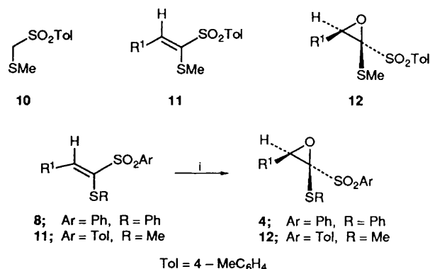
Scheme 2 Reagents and conditions: i, Bu'O 2 Li, THF, –78 to –18 °C.
