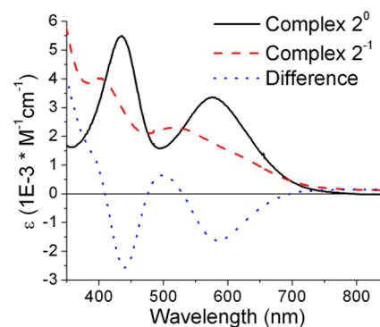
Figure 4. Reducing complex 2 by one electron ( 2 − , red dashed line) resulted in decreases in the absorbance of the neutral state ( 2 , black solid line). The difference between the 2 − and 2 spectra (blue dotted line) represents the contributions of 1 to the transient spectra in Figure 5.
