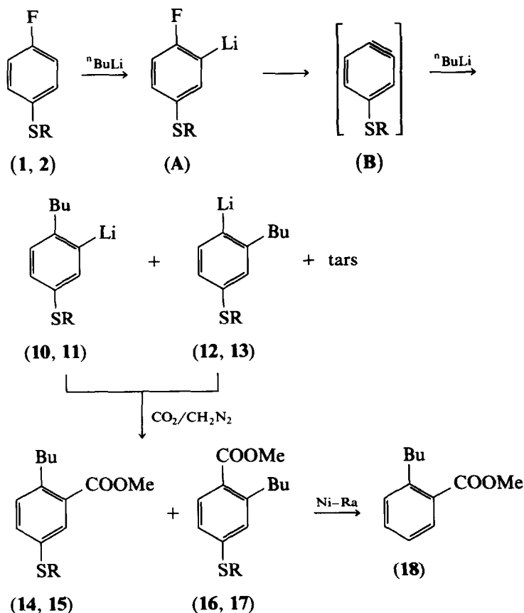
Scheme 2
