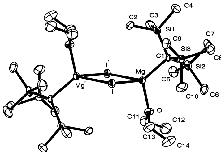
Fig. 5. Molecular structure of [\text{Mg}(\text{OEt}_2)\{\text{C}(\text{SiMe}_3)_3\}\text{I}]_2 ( 10 ).
