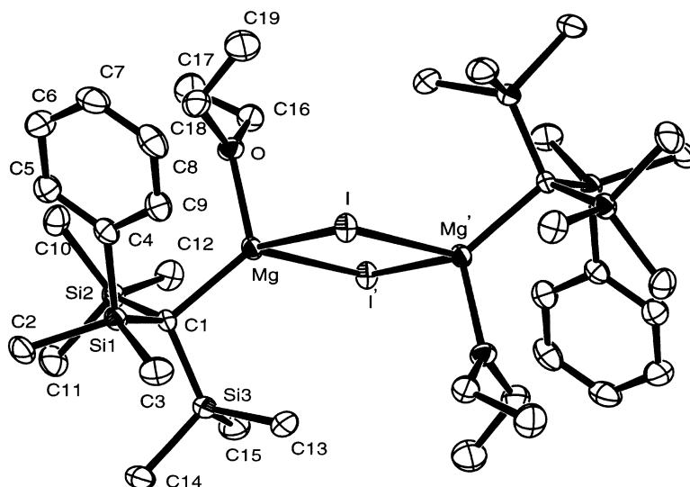
Fig. 6. Molecular structure of [\text{Mg}(\text{OEt}_2)\{\text{C}(\text{SiMe}_3)_2(\text{SiMe}_2\text{Ph})\}\text{I}_2] ( 11 ).
