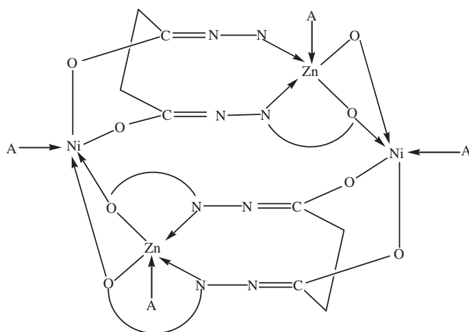
Figure 4. Tentative structure of [\text{ZnNi}(\text{nsh})(\text{A})_2] .
