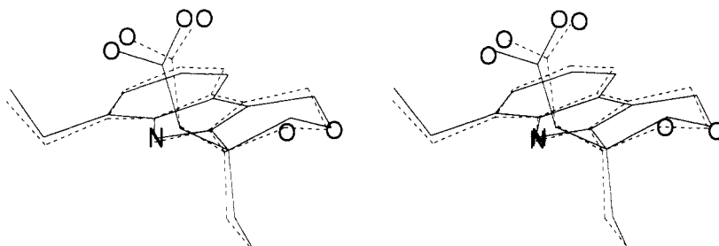
Figure 1. Stereoview of the overlap of etodolac (1) (---) and its pyrano[4,3- b ]indole isomer 7 (—).
