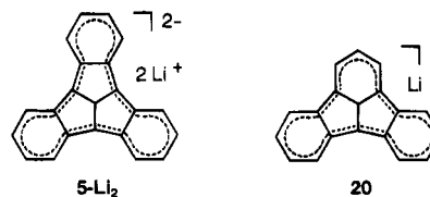
Figure 5. Charge distribution in 5-Li 2 and 20 .
