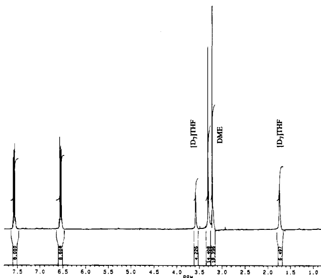
Figure 6. ^1\text{H} NMR spectrum of dilithium tribenzacepentalediide ( 5\text{-Li}_2 ) (250 MHz, [\text{D}_8]\text{THF} ) showing the line pattern of a single AA'XX' spin system for the 12 arene protons.
