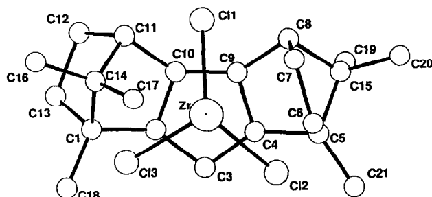
Fig. 2. Top view of the molecular geometry of complex 7a in the crystal.
