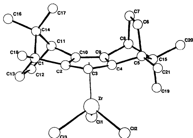
Fig. 1. A view of the molecular geometry of “(+)-(diborna-Cp)ZrCl 3 ” ( 7a ). Selected bond lengths (Å) and angles (deg): Zr–Cl(1) 2.358(1), Zr–Cl(2) 2.377(1), Zr–Cl(3) 2.372(1), Zr–C(2) 2.506(2), Zr–C(3) 2.453(3), Zr–C(4) 2.447(3), Zr–C(9) 2.577(3), Zr–C(10) 2.609(3), C(2)–C(3) 1.420(4), C(2)–C(10) 1.420(4), C(3)–C(4) 1.425(4), C(4)–C(9) 1.428(4), C(9)–C(10) 1.407(3), Cl(3)–Zr–Cl(2) 93.2(1), Cl(3)–Zr–Cl(1) 103.3(1), Cl(2)–Zr–Cl(1) 111.2(1). For additional structural data see Table 1.
