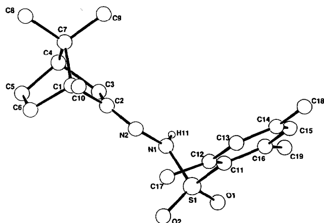
Fig. 3. Molecular structure of 2b .
