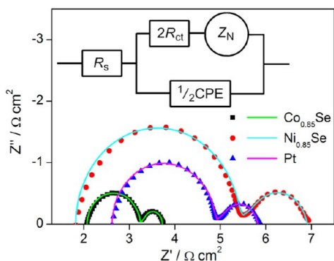
Figure 7. Nyquist plots for symmetrical cells fabricated with \text{Co}_{0.85}\text{Se} , \text{Ni}_{0.85}\text{Se} , and Pt CEs. The lines express fit results for corresponding EIS data, and the inset gives the equivalent circuit.
