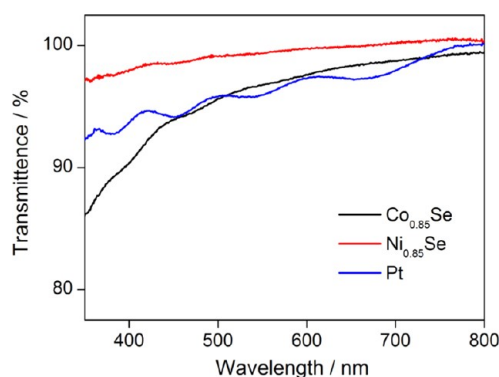
Figure 2. Optical transmittance spectra of \text{Co}_{0.85}\text{Se} , \text{Ni}_{0.85}\text{Se} , and Pt CEs.
