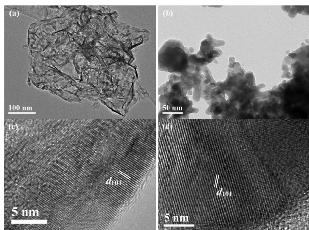
Figure 4. HRTEM images of as-synthesized \text{Co}_{0.85}\text{Se} (a,c) and \text{Ni}_{0.85}\text{Se} (b,d).
