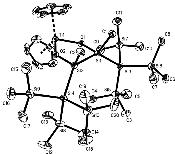
Fig. 3. Molecular structure of ( Z )- 7 in the crystal (ORTEP, 30% probability level, H-atoms omitted for clarity). Selected bond lengths [Å] and angles [°]: Ti1–O1 1.886(2), Ti1–O2 1.881(2), Si1–O1 1.652(2), Si2–O2 1.644(3), Si1–Si2 2.4404(15), Si2–Si4 2.3933(16), Si1–Si3 2.3898(16), O2–Ti1–O1 90.66(10), O1–Si1–Si2 94.40(9), O2–Si2–Si1 93.76(9), Si1–O1–Ti1 129.18(13), Si2–O2–Ti1 130.78(13), Si3–Si1–Si2 136.84(6), Si4–Si2–Si1 136.29(6), O1–Si1–Si2–O2 5.20(13), Si2–Si1–O1–Ti1 11.95(17), O2–Ti1–O1–Si1 12.49(18), O1–Ti1–O2–Si2 6.52(19), Si1–Si2–O2–Ti1 1.40(18).
