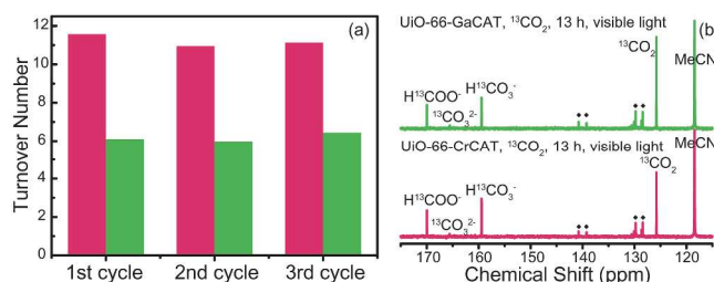
Fig. 3. (a) Photocatalytic ability of UiO-66-CrCAT (red) and UiO-66-GaCAT (green) over three cycles (6 h/cycle); (b) 13 C liquid NMR spectra of photocatalytic CO 2 reduction by UiO-66-CrCAT (red) and UiO-66-GaCAT (green) after 13 h reaction.
