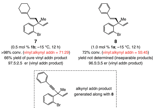
Scheme 4. NHC–Cu-Catalyzed EAS with Aryl Alkynes or Enynes Leads to Significant Amounts of Alkynyl Addition Products
