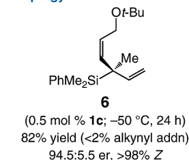
Scheme 4. NHC–Cu-Catalyzed EAS with Aryl Alkynes or Enynes Leads to Significant Amounts of Alkynyl Addition Products
