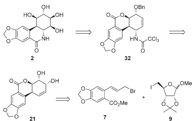
Scheme 5. Retrosynthesis: second-generation synthesis.
