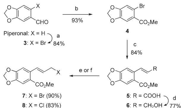
Scheme 2. a) Ref. [25]; b) NaClO 2 , NaH 2 PO 4 , acetone, H 2 O, then MeOH, H 2 SO 4 , 65°C; c) acrylic acid, Pd(OAc) 2 , Ph 3 P, Bu 3 N, toluene, 110°C; d) ClCO 2 Et, Et 3 N, THF, 0°C, then NaBH 4 , THF, H 2 O, 0°C; e) Ms 2 O, Et 3 N, LiBr, THF, –40°C → RT; f) MsCl, Et 3 N, LiCl, THF, –30°C → RT.
