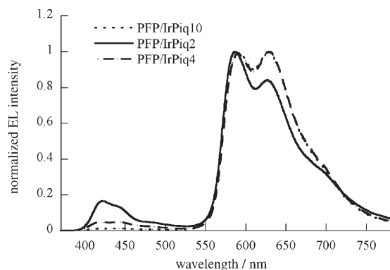
Figure 9. EL spectra of the devices fabricated from PFP/ IrPiq blends. Device structure: ITO/PEDOT:PSS (50 nm)/(PFP/ IrPiq)+PBD (30 wt %) (75 nm)/TPBI (50 nm)/Ba (4 nm)/Al (150 nm).
