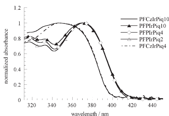
Figure 2. UV/Vis absorption spectra of charged Ir polymers in film.
