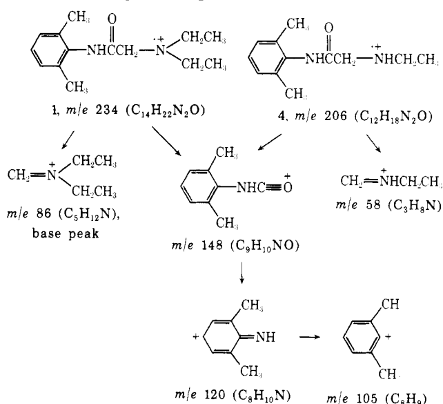
Scheme I. Mass Spectral Fragmentation Pattern for 1 and 4
