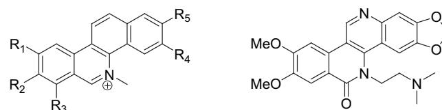
fagarone ( R_1 R_2 R_4 = \text{OMe} , R_3 = \text{H} , R_5 = \text{OH} ) nitidine ( R_1 R_2 = \text{OMe} , R_3 = \text{H} , R_4 R_5 = \text{OCH}_2\text{O} ) chelerythrine ( R_1 = \text{H} , R_2 R_3 = \text{OMe} , R_4 R_5 = \text{OCH}_2\text{O} ) sanguinarine ( R_1 = \text{H} , R_2 R_3 = \text{OCH}_2\text{O} , R_4 R_5 = \text{OCH}_2\text{O} )
