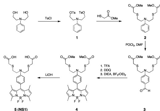
Scheme 1. Synthesis of Nickelsensor-1 (NS1)
