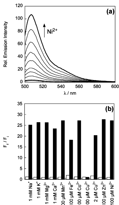
Figure 1. (a) Fluorescence response of 2 \mu\text{M} NS1 to \text{Ni}^{2+} . Spectra shown are for \text{Ni}^{2+} concentrations of 0, 2, 5, 10, 15, 25, 35, 50, 75, 100 \mu\text{M} . Spectra were acquired in 20 mM HEPES, pH 7.1, with 488 nm excitation. (b) Fluorescence responses of 2 \mu\text{M} NS1 to various metal ions. Bars represent the final ( F_i ) over the initial ( F_x ) integrated emission. Spectra were acquired in HEPES, pH 7.1. White bars represent the addition of the competing metal ion to a 2 \mu\text{M} solution of NS1. Black bars represent addition of 100 \mu\text{M} \text{Ni}^{2+} to the solution. Excitation was provided at 488 nm, with emission integrated over 498–700 nm.
