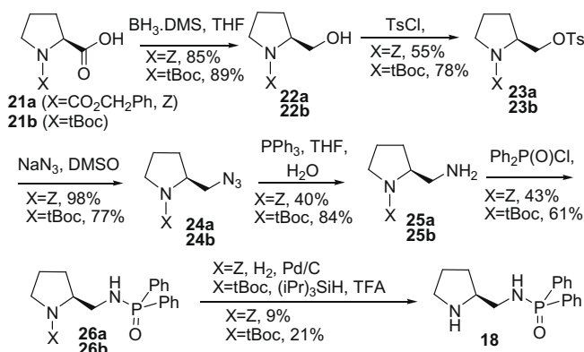
Scheme 2. Synthesis of 18 .
