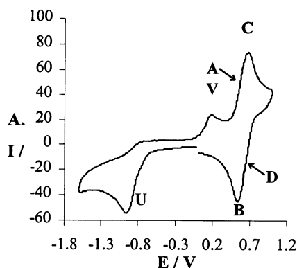
Fig. 4. Cyclic voltammogram of 20 at 200 mV s -1 .
