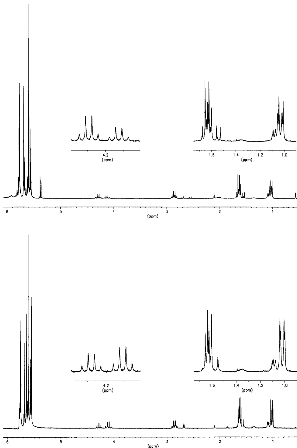
Fig. 1. ^1\text{H} NMR spectra of the mixture of monocarbonylation products trans - 10 and cis - 10 obtained from the 1.5 : 1 (top) and 1 : 1.7 mixtures (bottom) of the diastereomeric ( \eta^2 -acetaldehyde)zirconocene dimers trans - 9 and cis - 9 .
