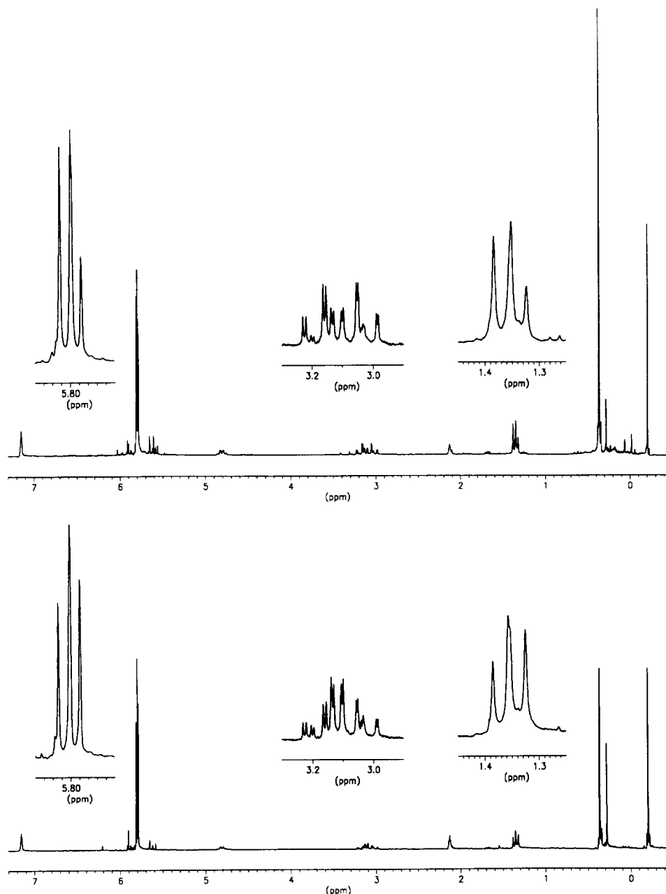
Fig. 3. 1 H NMR spectra of the mixture of diastereomeric bis-insertion products trans -12a and cis -12a obtained upon reacting the 1.5:1 (top) and 1:1.7 (bottom) mixtures of trans -9 and cis -9 with CNCH 2 SiMe 3 (in benzene- d 6 ).
