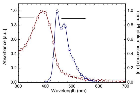
Fig. 3. UV–vis absorption and photoluminescence ( \lambda_{\text{exc}}=370 nm) of PBTA in THF solution.
