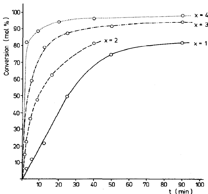
Fig. 1. Rate of formation of \text{Br}^- in the reaction between octyl bromide and the complex base [\text{BuLi} + x \text{ t-PenONa}] depending on x . For reaction conditions see Table 1.
