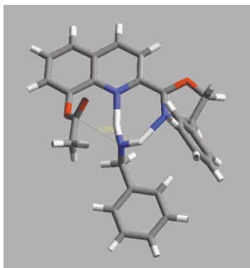
Figure 1. The hydrogen bonding complex between 8-acetoxy 2-oxazolinylquinoline and benzylamine has been minimized using the Cerius 2 ® package. The hydrogen bond between NH...N (quinoline) is 2.1 Å long and NH...N (oxazoline) is 1.9 Å long.
