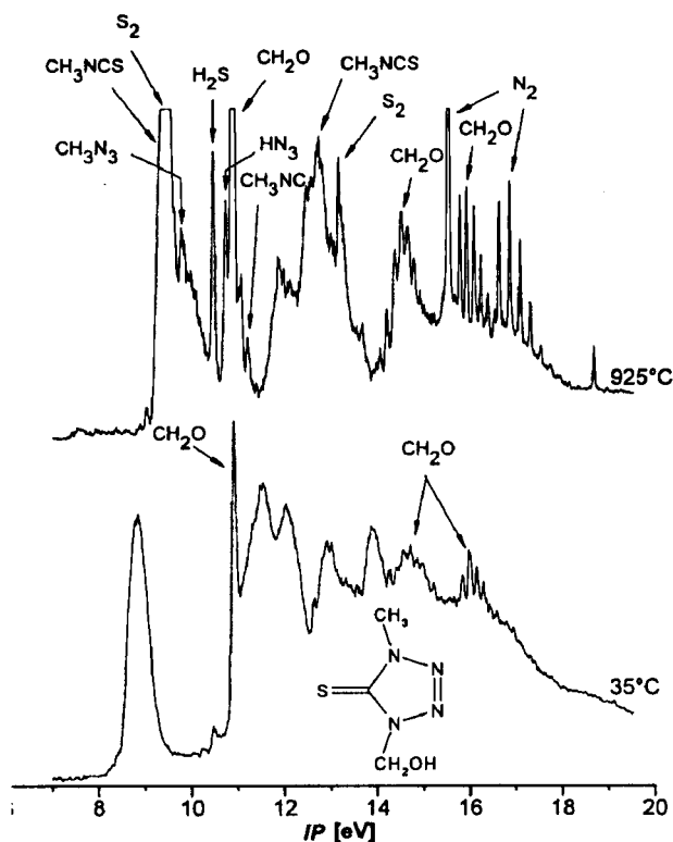
Figure 7. Photoelectron spectrum of tetrazolinethione 14 measured at different temperatures.
