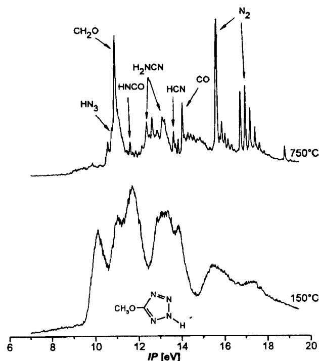
Figure 1. Photoelectron spectrum of tetrazole 1 measured at different temperatures.
