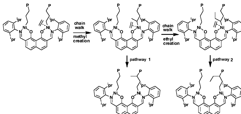
Scheme 2. Branch Formation Pathways in \text{FI}^2\text{-Ni}_2 Mediated Ethylene Homopolymerization
