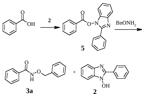
Probable mechanism and isolation of intermediate 5 .
