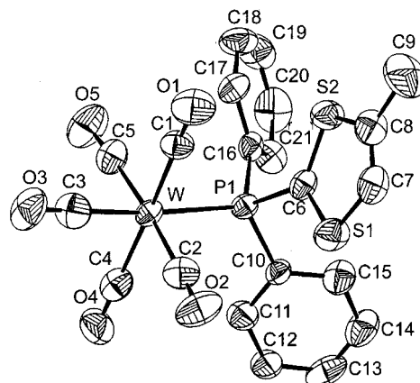
Figure 1. ORTEP drawing with 30% thermal ellipsoids and atom-numbering scheme for the cationic complex \text{W(CO)}_5[\text{PPh}_2\text{CSCHC(CH}_3\text{)S}]^+ ( 6 ).
