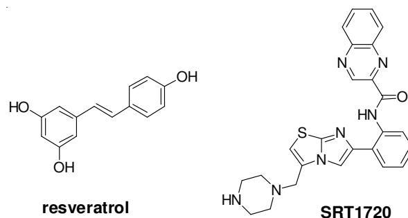
Fig. 1. Structures of the reported SIRT1 activators
