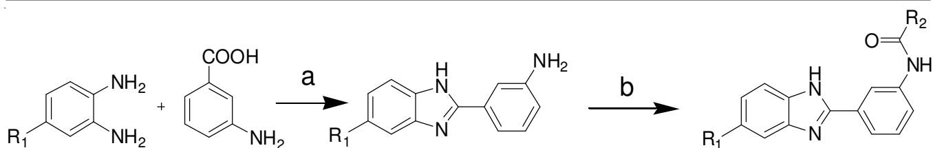
Scheme-I: Reagents and conditions: (a) PPA, 200 °C, 6 h (yield 85-93 %); (b) RCOOH, CH 2 Cl 2 , EDCI, DMAP, Et 3 N, 60 °C, 6 h (yield 32-86 %)
