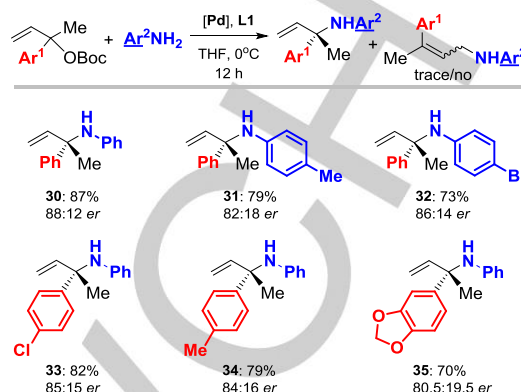
Figure 4. Scope in allylic precursors and anilines: allylic precursor (0.15 mmol) aniline reagent (0.23 mmol), Pd_2(dba)_3 \cdot CHCl_3 (1.25 mol %), L1 (5 mol %), THF (0.2 mL), 0°C, open to air, 12 h. Isolated yields are reported.
