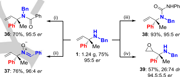
Figure 5. Various conversions of allylic amine 1 : (i) Benzoyl chloride (1.3 equiv), NEt_3 (5 equiv), CH_2Cl_2 , rt, 50 min. (ii) m -CPBA (2.3 equiv), CH_2Cl_2 , 0-rt, 2 h. (iii) Phenyl isocyanate (1.3 equiv), NEt_3 (10 equiv), CH_2Cl_2 , rt, 10 min. (iv) TsOH (1.02 equiv), m -CPBA (1.2 equiv), CH_2Cl_2 , 0-rt, 3 h; see SI for details.
