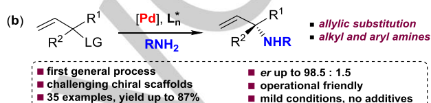
Scheme 1. Enantioselective synthesis of \alpha,\alpha -disubstituted allylic amines. LG stands for leaving group.
