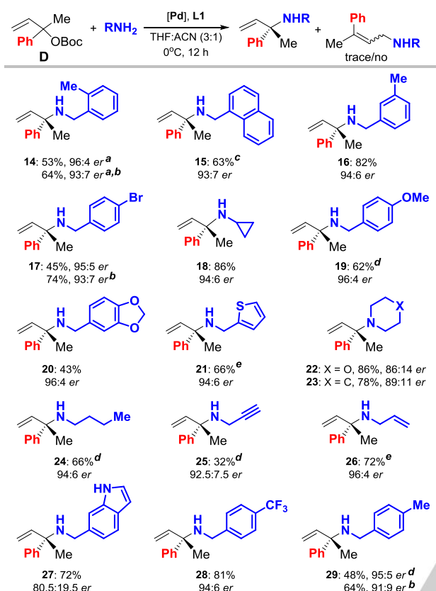
Figure 3. Scope in aliphatic amines: allylic precursor D (0.15 mmol), amine (0.17 mmol, 1.1 equiv), Pd_2(dba)_3 \cdot CHCl_3 (2 mol %), L1 (10 mol %), THF/ACN (3:1; 0.35 mL), 0°C, open to air, 12 h; isolated yields are reported and the er values were determined by UPC2. [a] 24 h. [b] CsF (3 equiv) was added, THF/ACN/H 2 O (3:1:0.4). [c] Amine (1.5 equiv). [d] 36 h. [e] The er values were determined by using a chiral shift reagent (SI for details).
