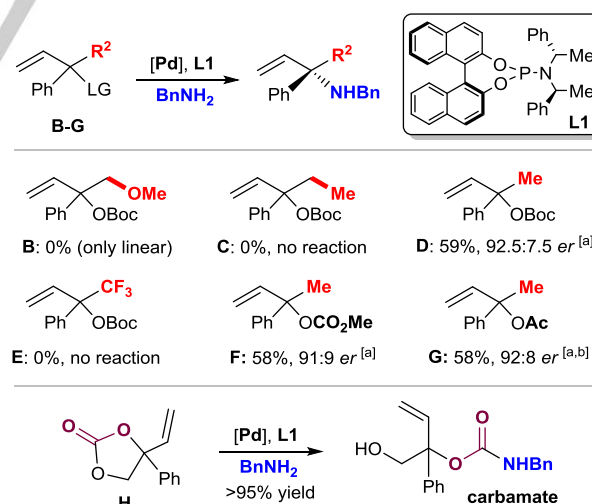
Figure 1. Preliminary screening of allylic precursors: B–G and H (0.15 mmol), BnNH 2 (0.23 mmol, 1.5 equiv), THF (150 \mu L), Pd 2 (dba) 3 ·CHCl 3 (3.5 mol %), L1 (14 mol %), open to air, rt, 12 h. [a] Isolated yield, er determined by UPC2 (see Supporting information (SI) for details). [b] 36 h.
