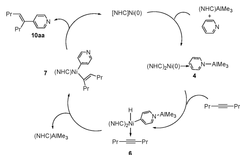
Scheme 2. Plausible Mechanism
