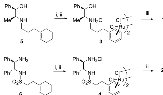
Scheme 1 a
