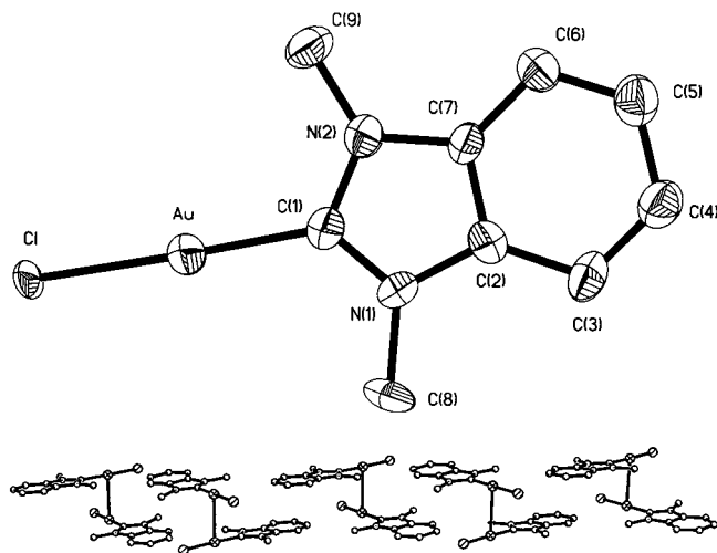
Figure 1. (a, top) ORTEP diagram (50% probability ellipsoids) of [\text{Au}(\text{Me}_2\text{-bimy})\text{Cl}] in the crystal state. Selected bond lengths (Å) and angles (deg): Au–Au, 3.1664(10); Au–C(1), 1.985(11); Au–Cl, 2.338(2); C(1)–N(1), 1.311(14); C(1)–N(2), 1.38(2); C(2)–N(1), 1.394(14); C(7)–N(2), 1.401(14); C(1)–Au–Cl, 178.1(3); N(1)–C(1)–N(2), 107.6(10); C(1)–Au–Au(1), 89.1(4). (b, bottom) Polymeric chain of [\text{Au}(\text{Me}_2\text{-bimy})\text{Cl}] , showing the \text{Au}^{\text{I}}\text{--Au}^{\text{I}} interaction and ring–ring \pi -stacking.
