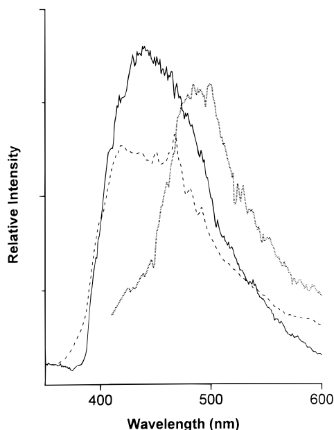
Figure 6. Emission spectra of [Au(Me 2 -bimy)(SPh)]: (a, solid line) at room temperature upon excitation at 315 nm; (b, dashed line) at 77 K upon excitation at 315 nm; (c, dotted line) at 77 K upon excitation at 390 nm.
