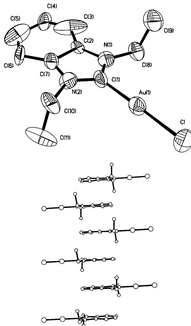
Figure 2. (a, top) ORTEP diagram (50% probability ellipsoids) of [\text{Au}(\text{Et}_2\text{-bimy})\text{Cl}] in the crystal state. Selected bond lengths (Å) and angles (deg): Au–C(1), 2.01(3); Au–Cl, 2.297(7); C(1)–N(1), 1.33(3); C(1)–N(2), 1.30(4); C(2)–N(1), 1.38(4); C(7)–N(2), 1.40(3); C(1)–Au–Cl, 179.5(8); N(1)–C(1)–N(2), 109(2). (b, bottom) Neighboring pairs of [\text{Au}(\text{Et}_2\text{-bimy})\text{Cl}] , showing the ring–ring \pi -stacking.
