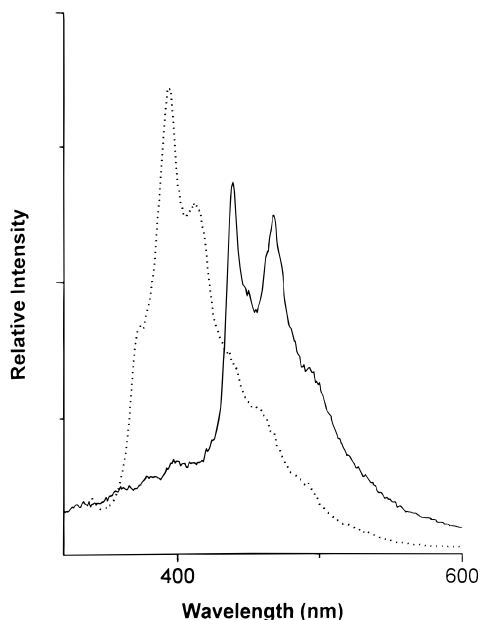
Figure 7. Emission spectra of [Au(R 2 -bimy) 2 ](PF 6 ) upon excitation at 290 nm: (a, solid line) R = Me; (b, dotted line) R = Et.
