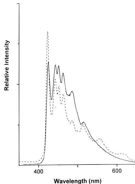
Figure 5. Emission spectra of [Au(R 2 -bimy)(C≡C)Ph] measured in the solid state at room temperature: (a, solid line) R = Me; (b, dashed line) R = Et. Excitation at 350 nm.
