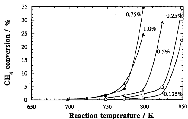
Figure 1. \text{CH}_4 conversion variation at different \text{NO}_2 concentration as a function of reaction temperature. Reaction gas: \text{CH}_4 (55.6%) + \text{O}_2 (27.7%) + \text{NO}_2 in He (balance). Flow rate: 120 mL/min.
