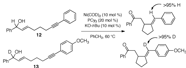
Scheme 4. Crossover Experiments
