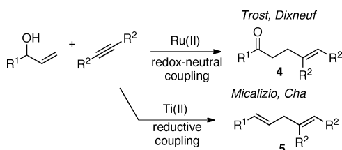
Scheme 2. Couplings of Allylic Alcohols and Alkynes
