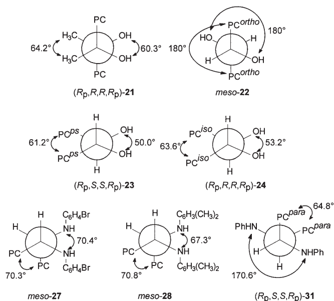
Figure 8. The conformations and characteristic torsion angles for diols and diamines in the crystal (PC: [2.2]paracyclophan-4-yl; PC ortho : 5-methoxy[2.2]paracyclophan-4-yl; PC ps : 12-methoxy[2.2]paracyclophan-4-yl; PC iso : 13-methoxy[2.2]paracyclophan-4-yl; PC para : 7-methoxy[2.2]paracyclophan-4-yl).
