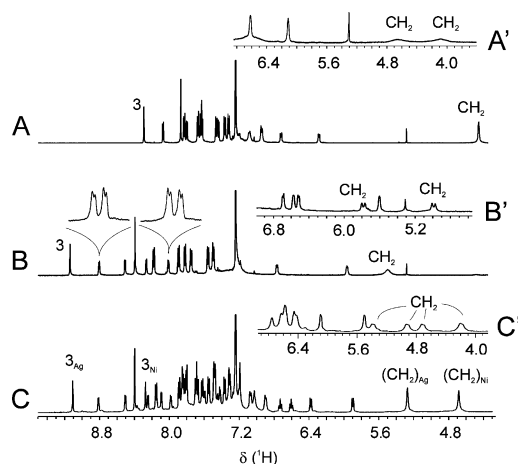
Figure 1. Low-field parts of the 1 H NMR spectra (500 MHz, CDCl 3 ) of 5 (A), 6 (B), and 13 (C) taken at 298 K. The expansions of two of the β-pyrrole resonances (components of an AB system) in trace B present signal splitting due to proton coupling with 107,109 Ag nuclei ( 4 J = 1.1 Hz). Insets A', B', and C' show fragments of the 1 H NMR spectra of 5 , 6 , and 13 , respectively, recorded in overcooled CDCl 3 at 203 K.
