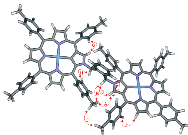
Figure 2. NOESY spectrum (top, 500 MHz, overcooled CDCl 3 , 203 K) and an energy-minimized model of 6 (bottom). The cross-peak assignments in the map (A–H) indicate interprotonic interaction marked on the model by curved arrows.
