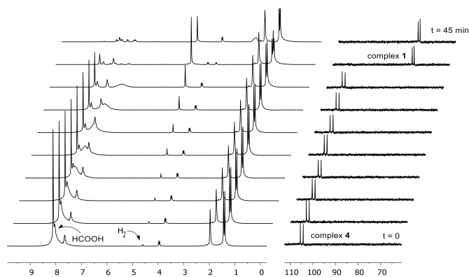
Scheme 3. Reactivity of Rh I complex 1 toward 10 molar equiv of HCOOH.
