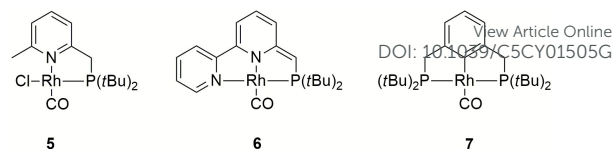
Figure 6. Other Rh ^I complexes that were studied in the dehydrogenation of formic acid.
